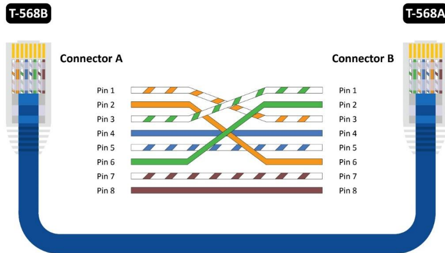
CROSSOVER WIRING (On Request)
