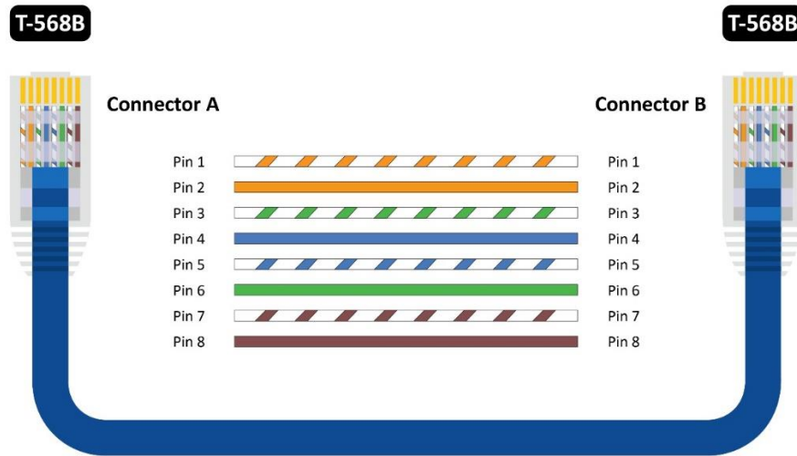
STRAIGHT-THROUGH WIRING (Nexconec Standard)
