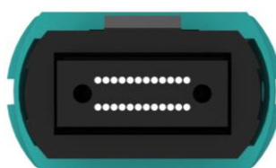
24 Fiber MTP/MPO
